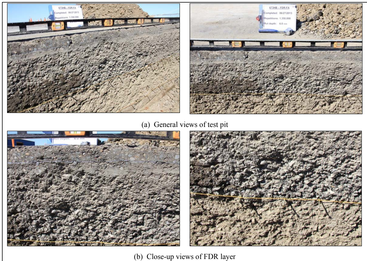
Figure 8.4: 673HB: Test pit photographs.
